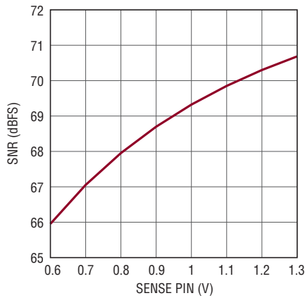
LTC2144-12: SNR vs SENSE, f_{IN} = 5\text{MHz} , -1dBFS
