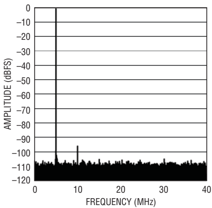
LTC2143-12: 64k Point FFT, f_{IN} = 5\text{MHz} , -1dBFS, 80MSPS
