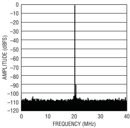
LTC2143-12: 64k Point FFT, f_{IN} = 140\text{MHz} , -1dBFS, 80MSPS
